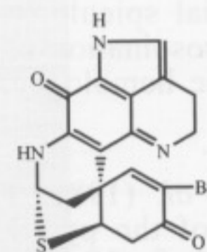
37 Discorhabdin A
