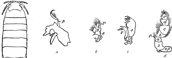
FIG. 5. 1 — a , Mandible of Cirolana borealis ; p , palpus. b , Maxilla of the second pair; 1 , first joint; 2 , second joint; l 2 , lobe of the second joint; 3 , third joint; l 3 , lobes of the third joint. c , Maxilla of the first pair; 1 , first joint; l 1 , lobe of the first joint; 2 , second joint; 3 , third joint. d , Maxilliped; 1 , first joint; ep , epignath; 2 , second joint; l 2 , lobe of the second joint; a , b , c , d , e , palpus.
