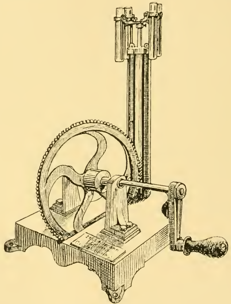
FIG. 250.—LOHMANN'S HAND-CENTRIFUGE.
