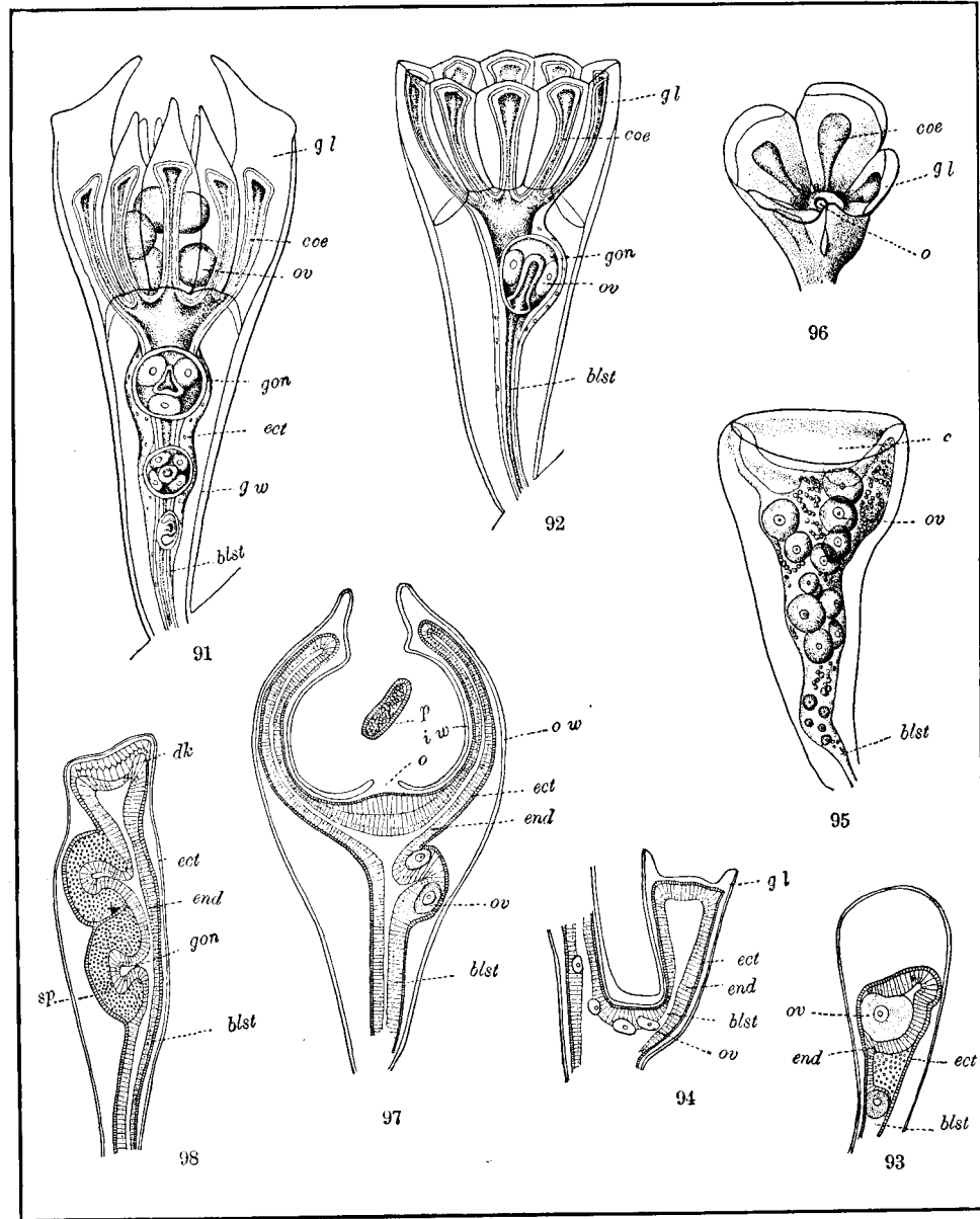
THE GONOSOME OF DIPHASIA. (Figs. 91 and 92 after Allman.)
