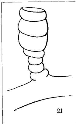
Fig. 21.—Very young hydrotheca of Sertularella rugosa , showing radial symmetry.
