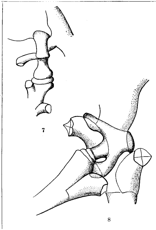
THE ANASTOMOSIS OF BRANCHES IN DICTYOCLADIUM.
