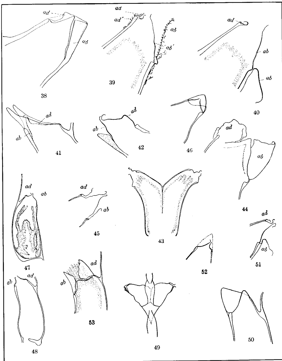
ENDS OF HYDROTHERE, GREATLY MAGNIFIED, TO SHOW BIVALVE OPERCULA. ( ad , adcauline flap; ab , abcauline flap.)
