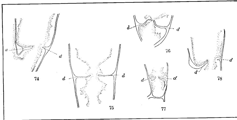
THE DIAPHRAGM OF THE SERTULARIIDE.
