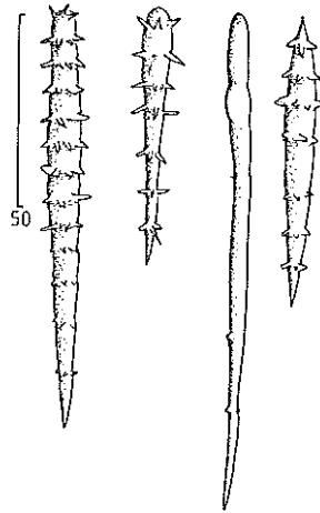
FIGURE 48. Agelas spec., variation of spicules.
