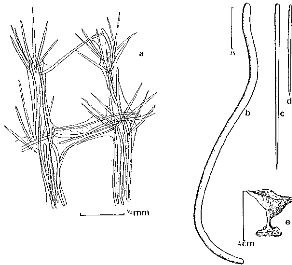
FIGURE 51. Phakellia folium , a. perpendicular section through peripheral region, b. sinuous strongyle, c. coring style, d. echinating small style, e. habit.
