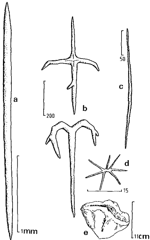
FIGURE 17. Poecillastra aspera , a. oxeote megasclere, b. orthotriaenes/dichotriaenes, c. roughened microxea, d. amphiaster, e. habit.
