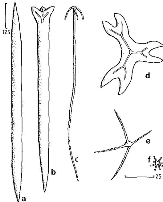
FIGURE 8. Stelletta cf. pumex , a. oxeote megasclere, b. plagiotriaene, c. anatriaene, d. dichotriaene, e. oxyaster, f. chiaster.
