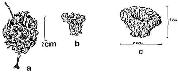
FIGURE 2. Habits of hexactinellid sponges, a. Aulocystis grayi , b. Cyrtaulon sigsbeeii , c. Dactylocalyx puniceus .
