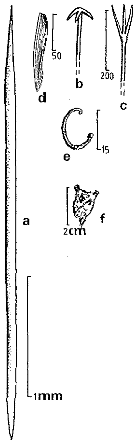
FIGURE 20. Cinachyra arenosa n. sp., a. oxeote megasclere, b. anatriaene, c. protriaene, d. trichodragma, e. sigmaspire, f. habit of holotype.
