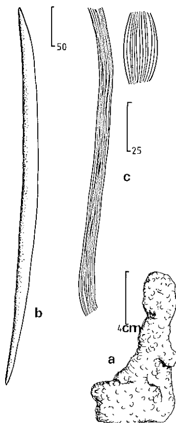
FIGURE 42. Epipolasis rea , a. habit, b. megasclere, c. trichodragmata in two size categories.
