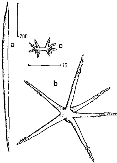
FIGURE 13. Asteropus simplex , a. oxeote megasclere, b. oxyaster, c. sanidaster.
