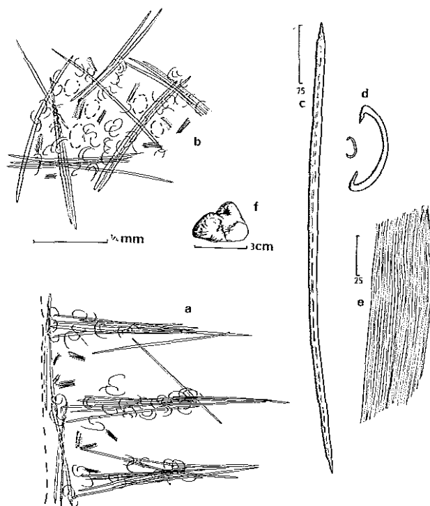
FIGURE 58. Biemna oxeata n. sp., a. perpendicular section of peripheral skeleton, b. tangential view of ectosomal skeleton, c. megasclere, d. sigmata in two size categories, e. trichodragma, f. habit.
