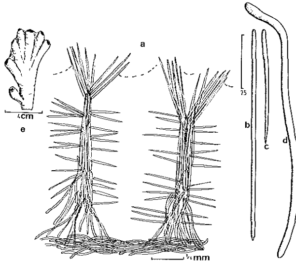
FIGURE 52. Auletta sycimularia , a. perpendicular section through peripheral skeleton, b. style of peripheral brushes and columns, c. echinating small style, d. sinuous strongyle of central axis, e. habit.
