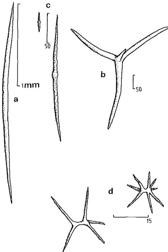
FIGURE 16. Poecillastra sollasi , a. oxeote megasclere, b. orthotriaene, c. roughened microxea, in two size categories, d. amphiasters.
