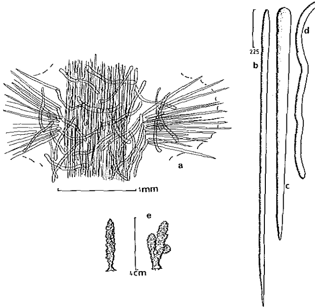
FIGURE 54. Bubaris rugosa , a. longitudinal section showing central axis of thick styles with enveloping sinuous strongyles and peripheral brushes of slender styles, b. slender style, c. thick style, d. sinuous strongyle, e. habits of characteristic specimens.
