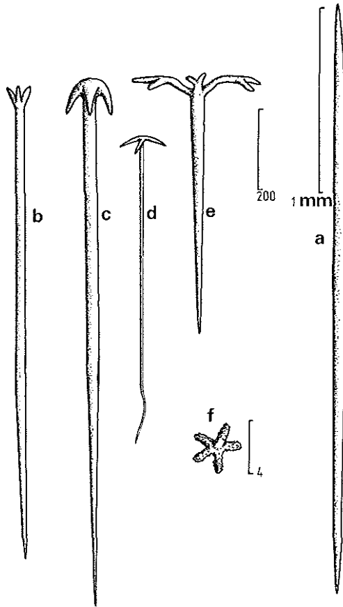
FIGURE 11. Stelletta spec., a. oxeote megasclere, b. protriaene, c. large thick anatriaene, d. thin anatriaene, e. dichotriaene, f. chiaster.
