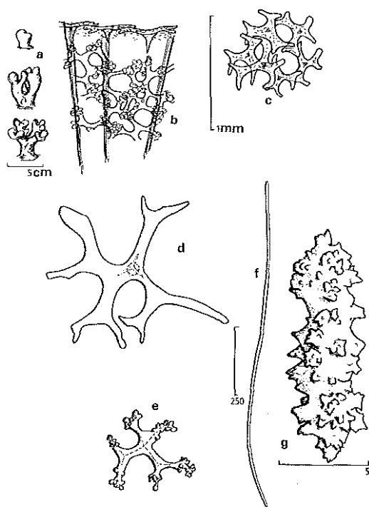
FIGURE 21. Theonella atlantica n. sp., a. habits of characteristic specimens, b. perpendicular section through peripheral skeleton, showing the position of the ectosomal phyllotriaenes, the desma reticulum and the supporting bundles of oxecotes, c. tangential view of ectosomal skeleton, d. ectosomal phyllotriaene, e. choanosomal desma, f. oxecote, g. acanthose microrhabd.
