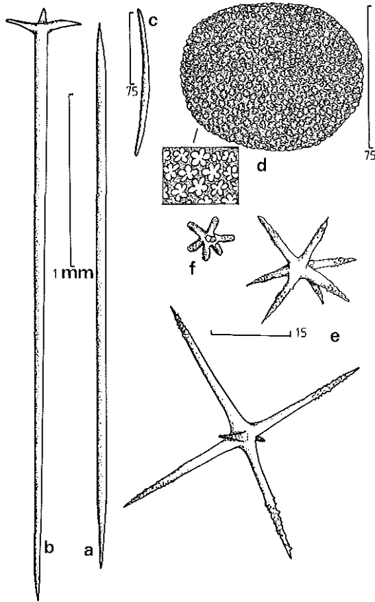
FIGURE 4. Geodia cf. megastrella , a. oxeote megasclere, b. orthotriaene, c. cortical small oxea, d. sterraster, with detail in inset, e. oxysphaerasters, f. strongylosphaeraster.
