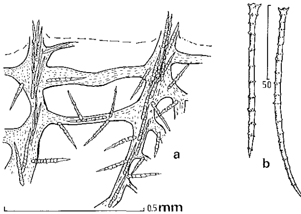
FIGURE 49. Agelas spectrum , a. perpendicular section through peripheral region, b. verticillate acanthostyles.
