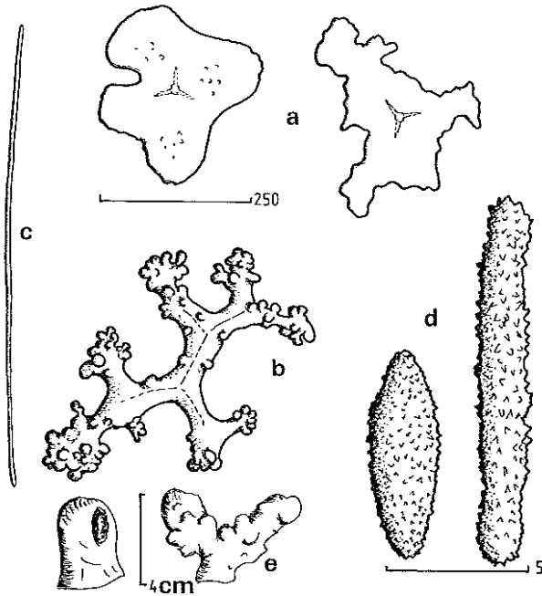
FIGURE 22. Discodermia polydiscus , a. ectosomal discotriaenes, b. desma, c. oxeote, d. acanthose microxea/microrhabd, e. habits of characteristic specimens.
