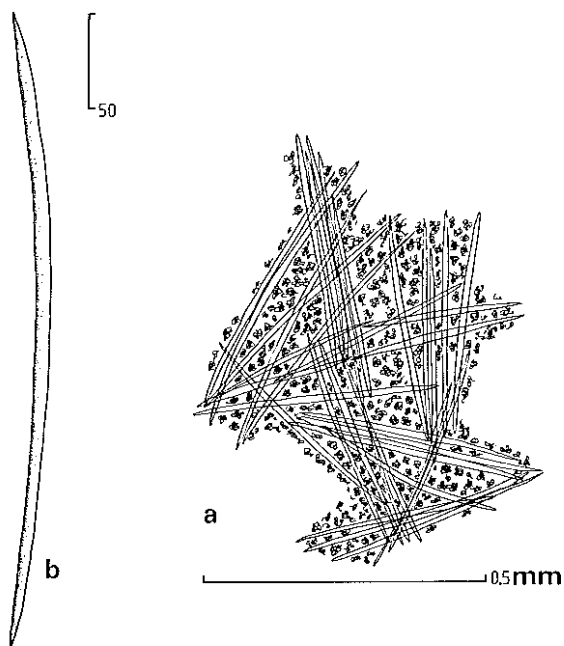
FIGURE 44. ? Halichondria ruetzleri n. sp., a. tangential view of ectosomal skeleton including heavy pigmentation of dermis, b. spicule.
