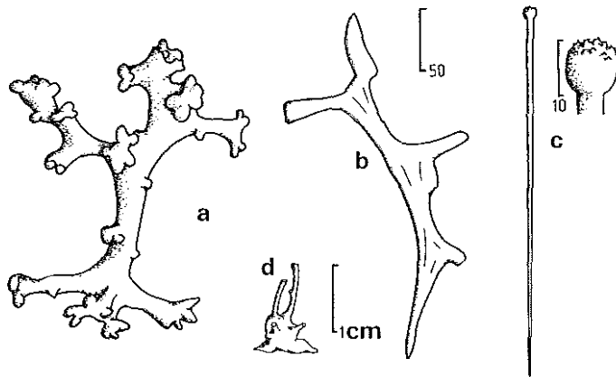
FIGURE 31. Siphonidium ramosum , a, choanosomal desma, b, ectosomal desma, c, tylostyle, with enlarged detail of rugose apex, d, habit.
