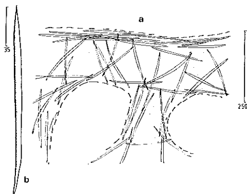
FIGURE 65. Calyx podatypa , a. perpendicular section through peripheral region, b. oxea.
