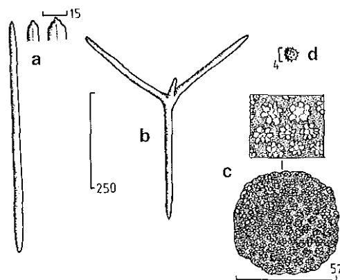
FIGURE 5. Caminus sphaeroconia , a. oxecote-strongylote megascleres (with enlarged variations of apices), b. orthotriaene, c. sterraster, with detail in inset, d. sphere.
