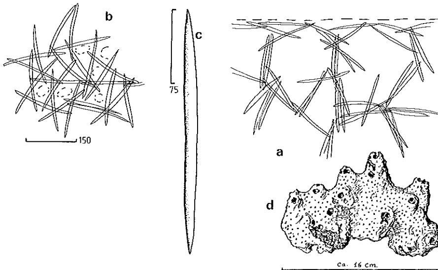
FIGURE 63. Xestospongia cf. rosariensis , a. perpendicular section through peripheral skeleton, b. tangential view of ectosome, c. oxea, d. habit.
