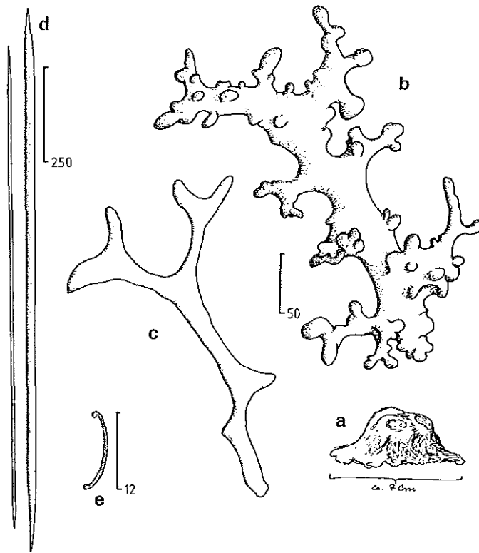
FIGURE 28. Amphibleptula madrepora , a. habit, b. desma, c. growth stage of desma, d. oxeotes, e. sigmaspire.
