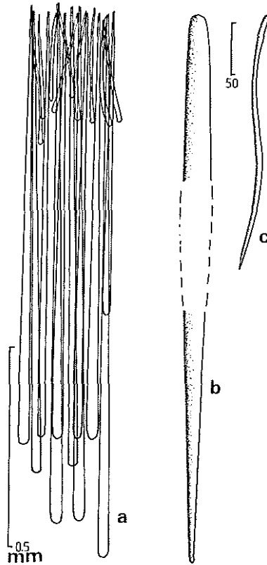
FIGURE 37. Aptos aaptos , a. perpendicular section through peripheral skeleton, b. megasclere, c. small style.
