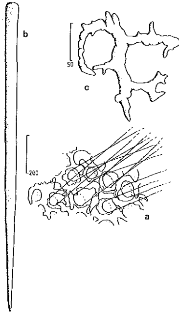
FIGURE 35. Lithobubaris tenens , a. architecture of the skeleton, with basal desmata and perpendicular huge styles, b. style, c. desma.
