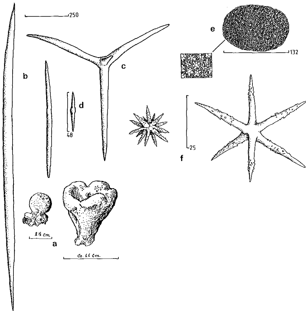
FIGURE 7. Pachymatisma geodiformis n. sp., a. habit, b. oxeote megascleres in two sizes, c. orthotriaene, d. centrotyle microxea, e. sterraster, with detail in inset, f. sphaeraster and oxyaster.
