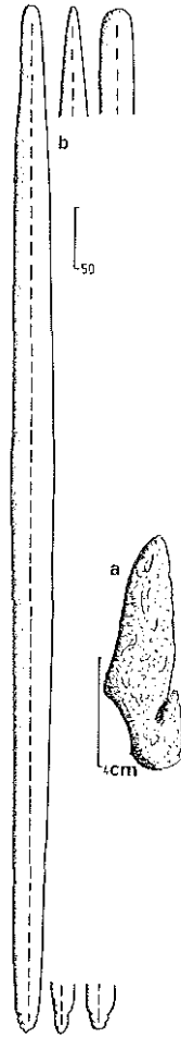
FIGURE 46. Leucophloeus lewisi n. sp., a. habit, b. style, including variation of apices.
