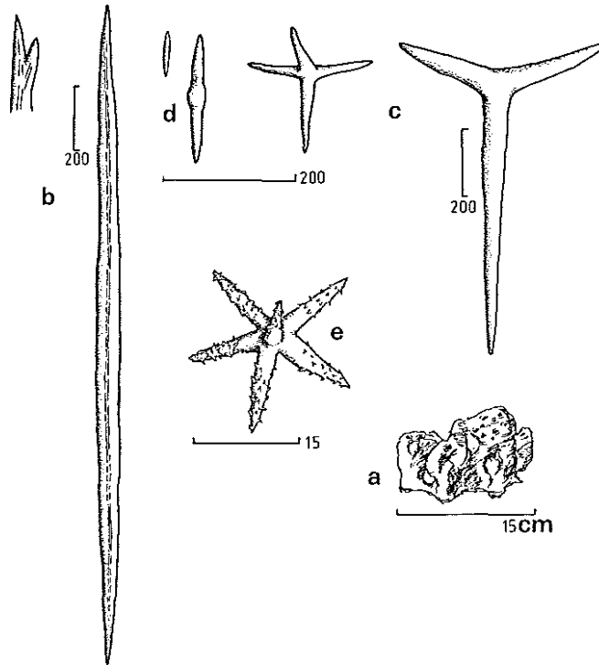
FIGURE 12. Penares mastoidea , a. habit, b. oxecote megasclere (with promonaene modification), c. ortho/plagiotriaenes, d. ectosomal small oxea in two size categories, e. oxyaster.
