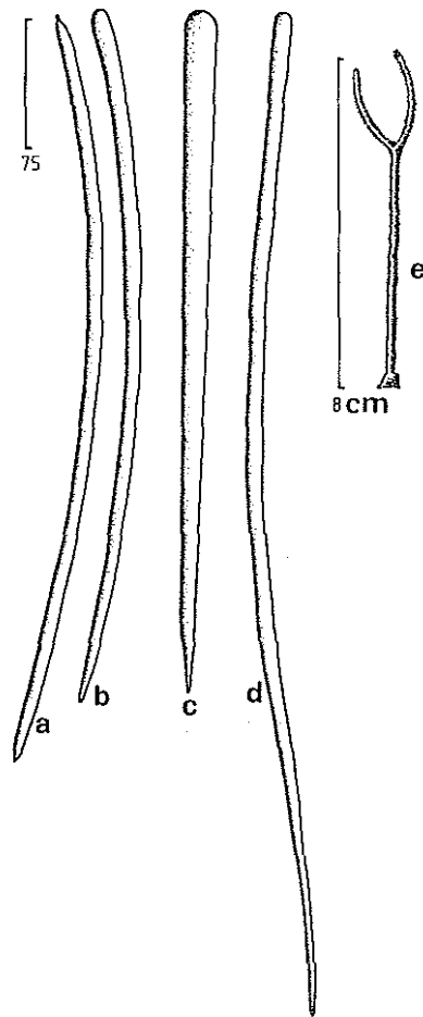
FIGURE 56. Raspailia cf. tenuis , a. oxea, b. style of the axial core, c. style of the radiating bundles, d. long style of the ectosomal brushes, e. habit.
