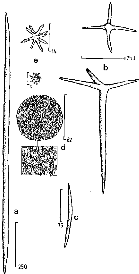
FIGURE 3. Geodia gibberosa , a. oxeote megasclere, b. orthotriaenes, c. cortical small oxea, d. sterraster, with detail in inset, e. sphaerasters (two size categories).
