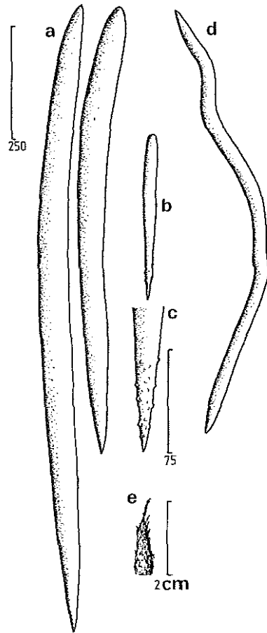
FIGURE 55. Bubaris flagelliformis n. sp., a. stylote megascleres, b. acanthose small styles, c. detail of spined basal part of small style, d. sinuous oxea, e. habit.
