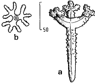
FIGURE 18. Thrombus kittoni , a. acanthotrichotriaene, b. dichotriaene growth stage.
