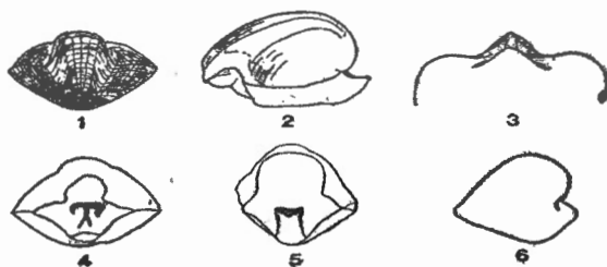
Fig. 4. Oxoplectia calhouni , Wilson. All natural size.
