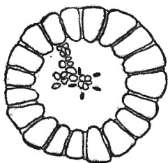
Fig. 3. Diagram of Cyclocystoides . From Narraway collection.
