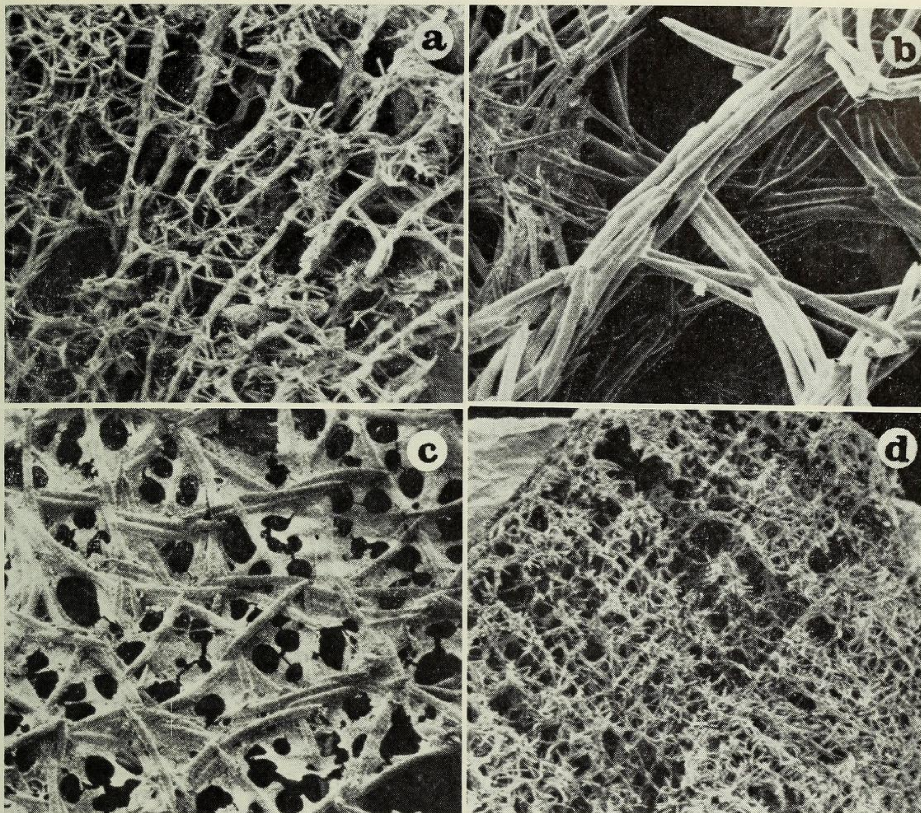
Fig. 4. a, Xestospongia trindanea : oxidized specimen showing reticulate pattern of multi-spicular tracts and confused arrangement of interstitial spicules (20 \times ); b, Xestospongia trindanea : large oxeads of multi-spicular tracts and smaller interstitial oxeads (lower right) (100 \times ); c, Adocia dubia : ectosomal tangential skeleton, ectosomal membrane and pores (125 \times ); d, Adocia dubia : oxidized specimen showing reticulate pattern and several growth lines (running from upper right to lower left) (20).
