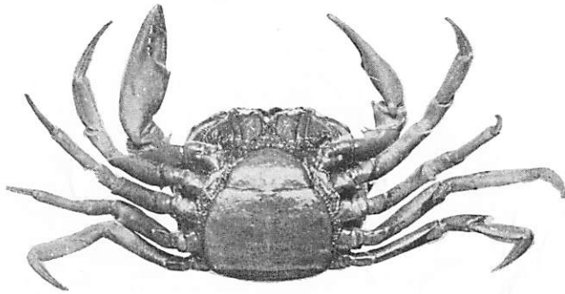
Fig. 2— T. (Dilocarcinus) pictus (Milne Edwards) face ventral ♀, tamanho natural
