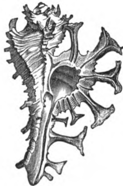
Fig. 138. — Rocher scorpion.
