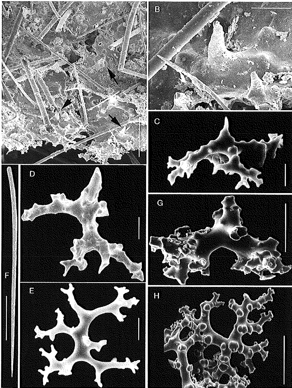
FIG. 2. — A–F, Desmanthus incrustans ; A, overview of uncleaned section of the type specimen, MNHN D.T. 1853 showing styles and rhabdomes of desmas II (arrows) protruding through the organic ectosome; B, detail of Fig. 2A showing the protruding rhabdomes of desmas II; C, Bonaire specimen ZMA 8491, desma II; D, Bonaire specimen ZMA 8491, desma II; E, Bonaire specimen ZMA 8491, desma I; F, Bonaire specimen ZMA 8491, style; G–H, Desmanthus topsenti , from type specimen SMF 1560; G, desma II; H, desma I. Scale bars: A, B, F–H, 100 µm; C–E, 10 µm.
