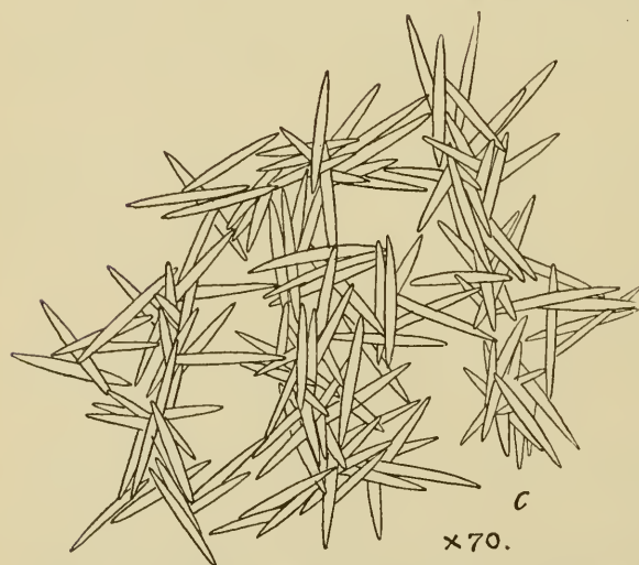
FIG. 4.—SPONGILLA CLEMENTIS. a, SKELETON SPICULES; b, GEMMULE SPICULE; c, FRAGMENT OF SKELETON.
