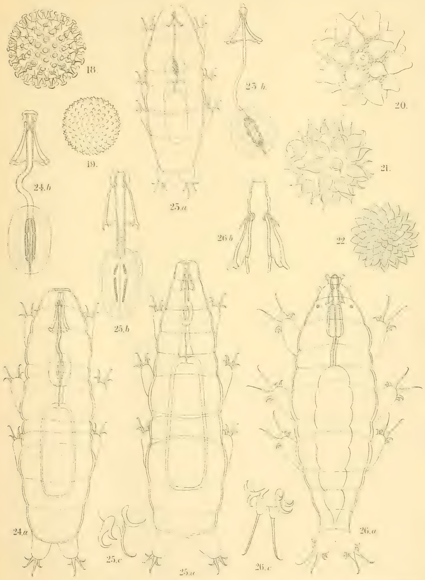
18, MACROBIOTUS HUFELANDI , C. Sch., Egg. 19, 20, 22, Eggs of MACROBIOTUS , sp? 21, M. ECHINOGENITUS , Richters. 23, DIPHASCON CHILENSE , Plate. 24 D. SPITZBERGENSE , Richters 25, D. ANGUSTATUM , n.sp. 26, MILNECIUM TARDIGRADUM , Doy
