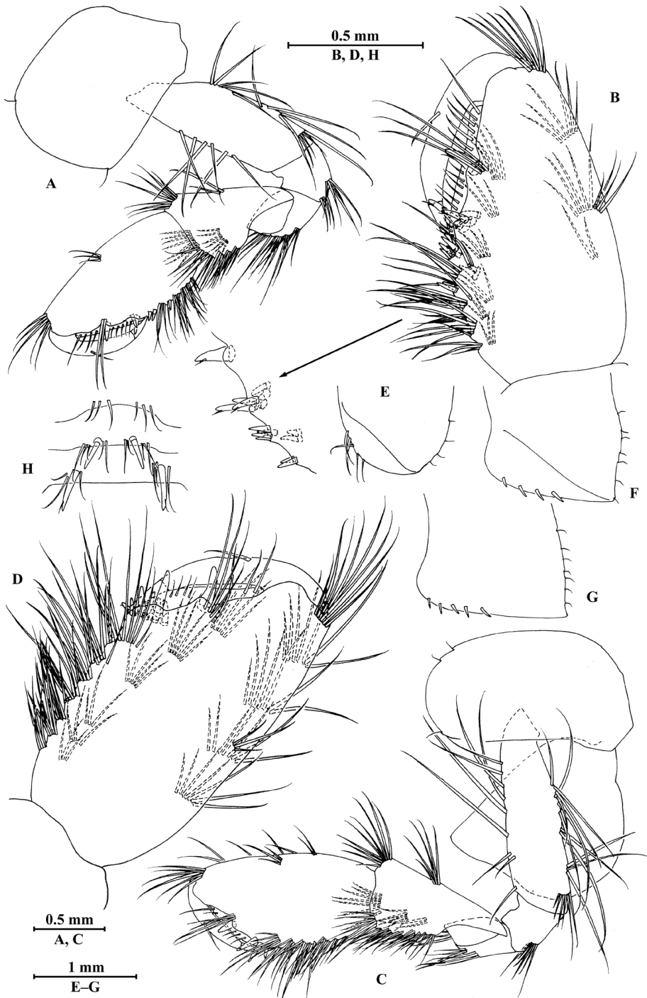
Figure 40. Gammarus caecigenus Hou & Li, sp. n., male holotype. A gnathopod I B propodus and dactylus of gnathopod I C gnathopod II D propodus and dactylus of gnathopod II E epimeral plate I F epimeral plate II G epimeral plate III H dorsal margins of urosomites I–III.
