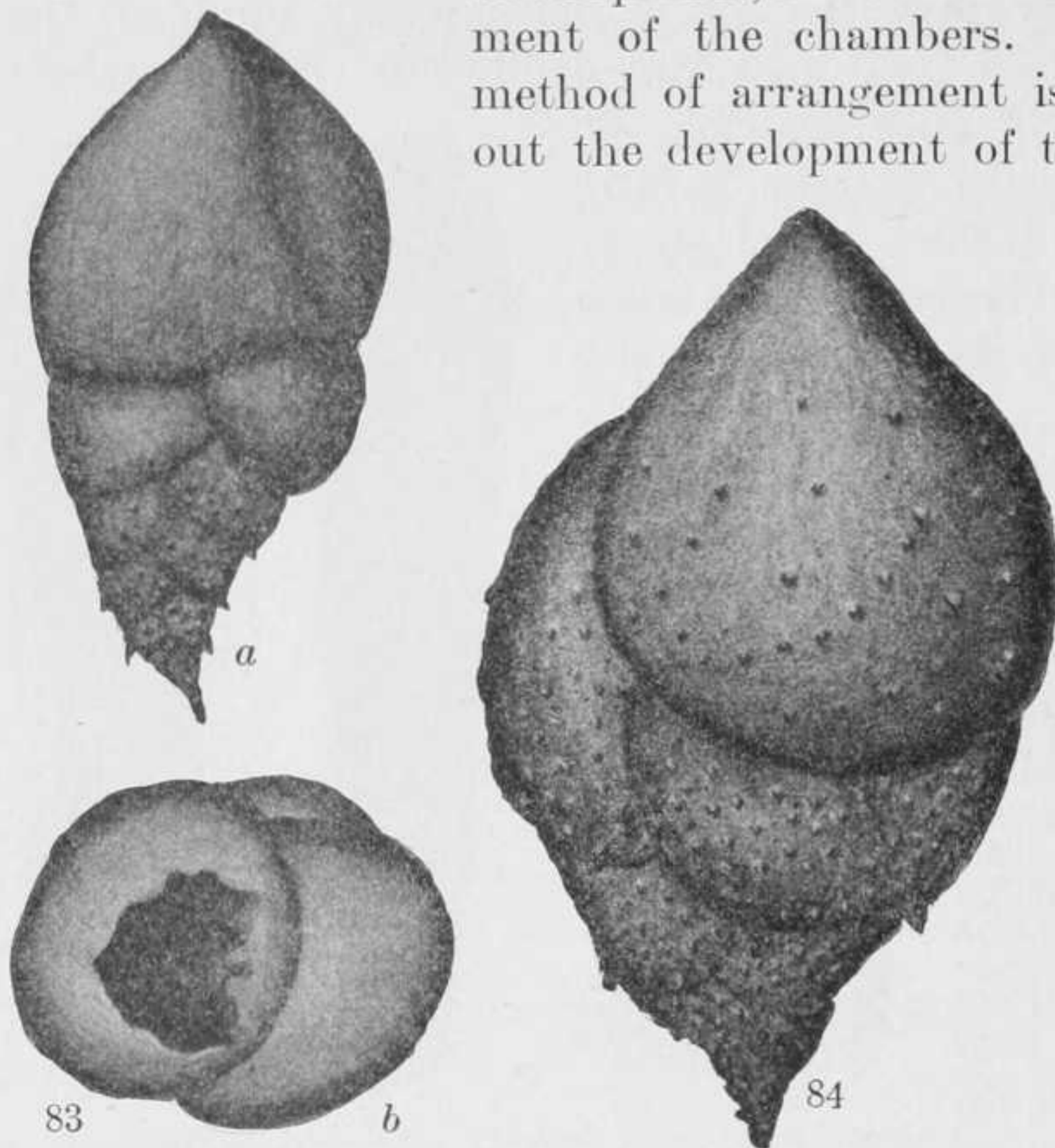
FIGS. 83-84.—PLEUROSATOMELLA SPINOSA. \times 75 . 83, a , FRONT VIEW; b , APERTURAL VIEW WITH THE UPPER END OF THE CHAMBER SLIGHTLY BROKEN AND JAGGED. 84, FRONT VIEW OF ANOTHER MORE INFLATED SPECIMEN.
