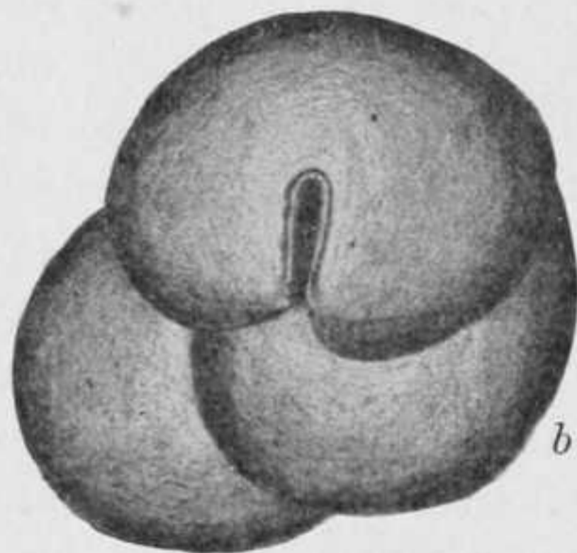
FIG. 136.— BULIMINA MARGINATA . × 150. a, FRONT VIEW; b, APERTURAL VIEW.
