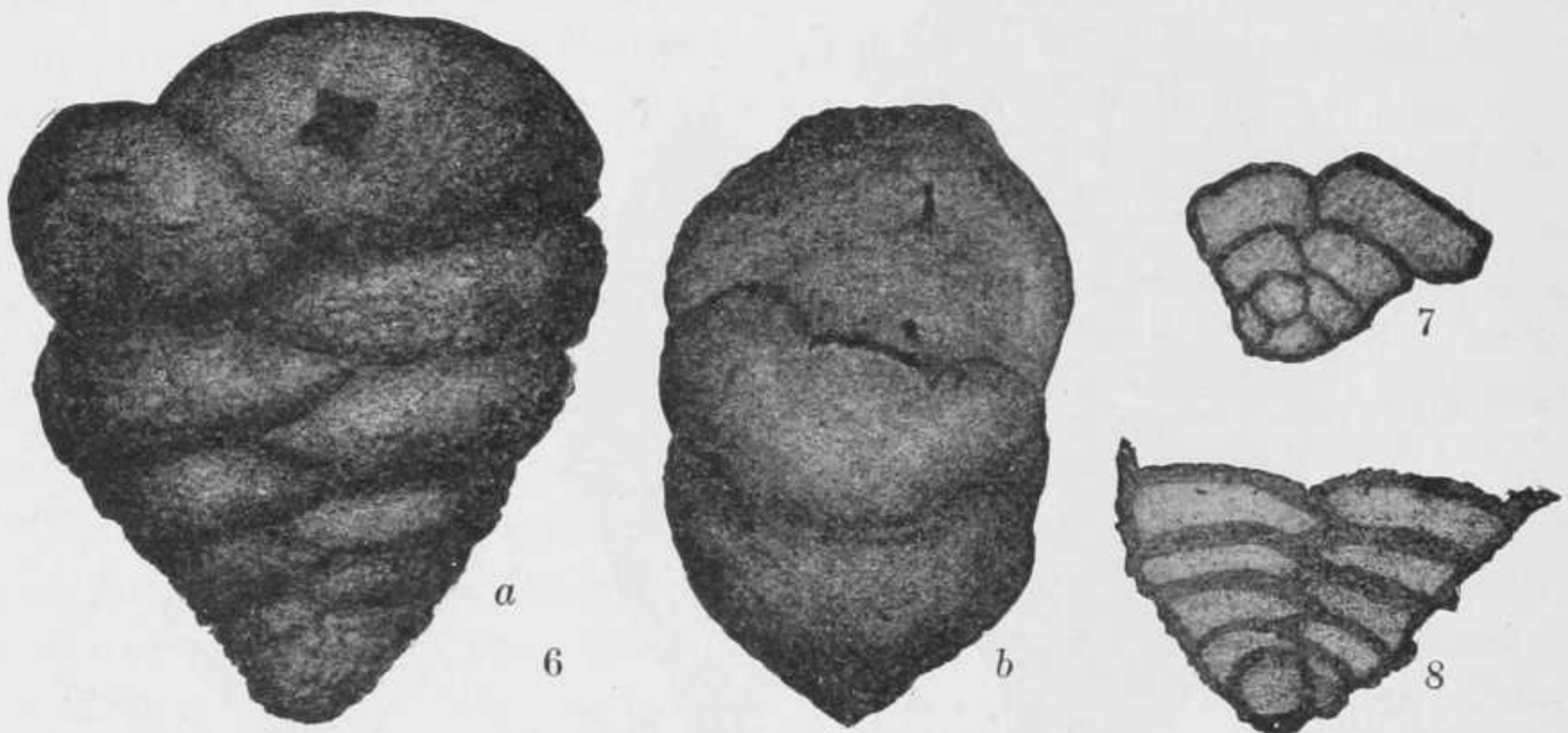
FIGS. 6-8.—TEXTULARIA GRAMEN. 6, a , SIDE VIEW; b , END VIEW. \times 60 . 7, MICROSPHERIC PROLOCULUM AND SUCCEEDING CHAMBERS VIEWED BY TRANSMITTED LIGHT, THE EARLY CHAMBERS FORMING A COILED GROUP HALFWAY AROUND THE PROLOCULUM. \times 150 . 8, MEGALOSPHERIC PROLOCULUM AND SUCCEEDING CHAMBERS, THE CHAMBERS FOLLOWING THE PROLOCULUM ASSUMING THE BISERIAL FORM AT ONCE WITHOUT TRACE OF COILING. SPECIMEN VIEWED BY TRANSMITTED LIGHT. \times 75 .
