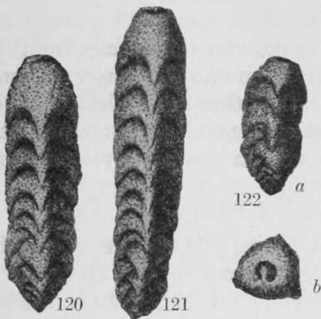
120-122.—CLAVULINA ANGULARIS \times 35 . 122, a, FRONT VIEW; b, APERTURAL VIEW (AFTER BRADY).
