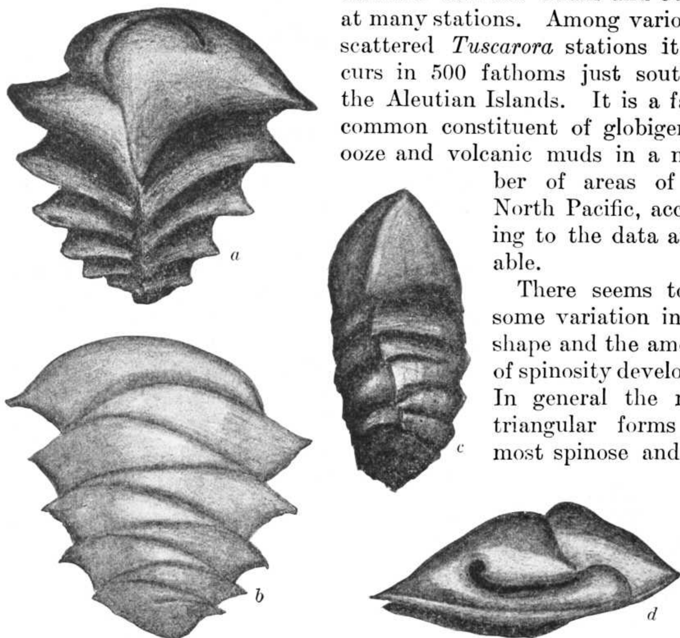
FIG. 155.— EHRENBERGINA SERRATA . \times 75 . a , VENTRAL VIEW; b , DORSAL VIEW; c , SIDE VIEW; d , APERTURAL VIEW.
