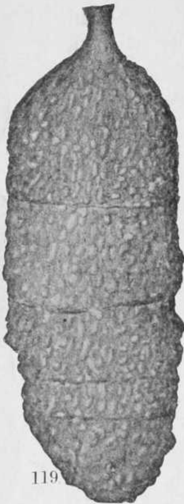
FIGS. 118-119.— CLAVULINA BRADYI . \times 30 . 118, a , END VIEW, WITHOUT TOOTH; b , FRONT VIEW OF TYPICAL SPECIMEN. 119, FRONT VIEW OF A PECULIARLY ROUGHENED SPECIMEN.
