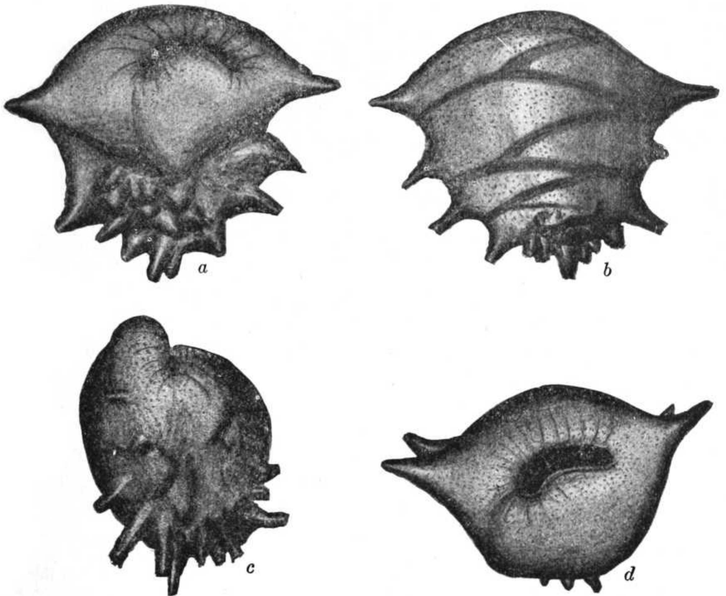
FIG. 156.—EHRENBERGINA HYSTRIX. \times 40 . a , VENTRAL VIEW; b , DORSAL VIEW; c , SIDE VIEW; d , APERTURAL VIEW.
