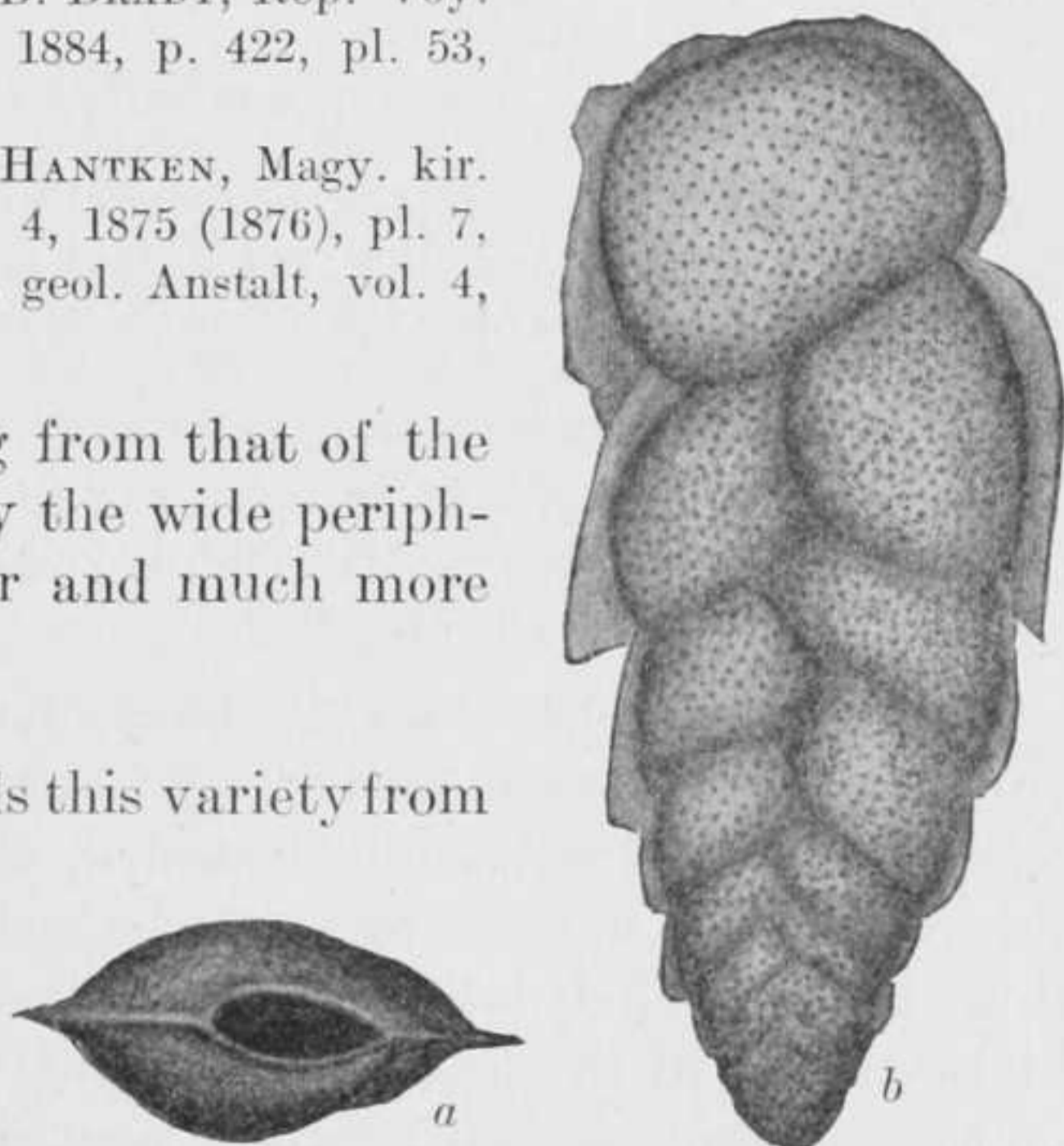
FIG. 57.— BOLIVINA BEYRICHI , VAR. ALATA . \times 60 . a , APERTURAL VIEW; b , FRONT VIEW.
