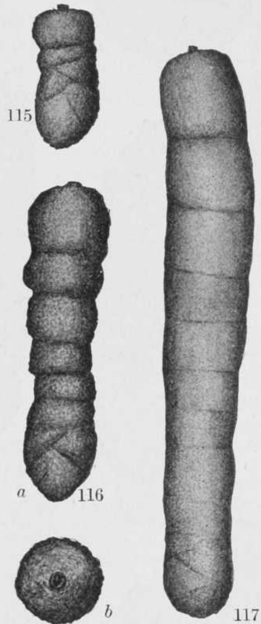
FIGS. 115–117.—CLAVULINA COMMUNIS. X 30. 115, YOUNG SPECIMEN WITH BUT TWO OF THE SECOND SERIES OF CHAMBERS DEVELOPED. 116, a , FRONT VIEW OF MEDIUM-SIZED SPECIMEN; b , END VIEW OF THE SAME. 117, ADULT SPECIMEN IN FRONT VIEW.
