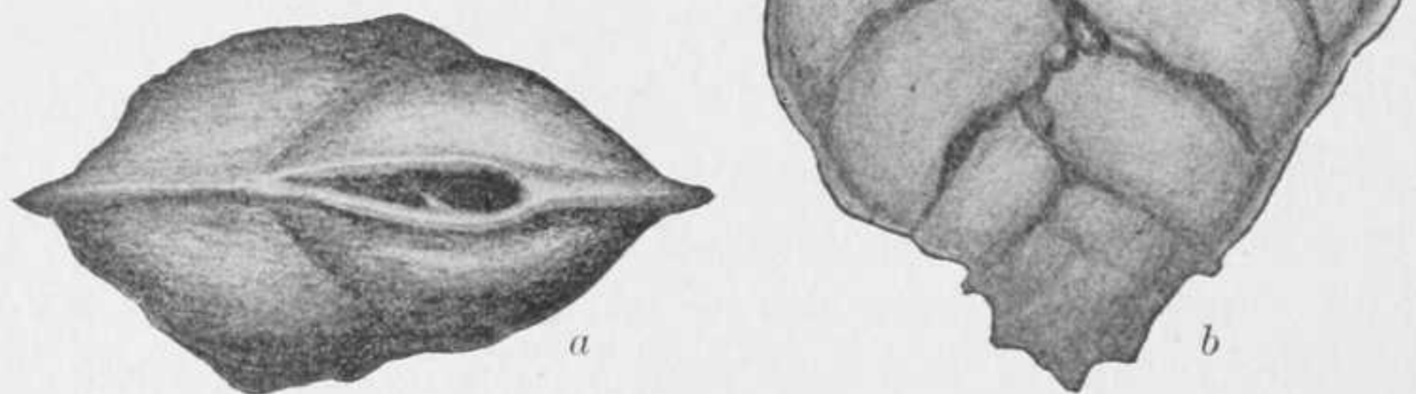
FIG. 63.— BOLIVINA SCHWAGERIANA . \times 65 . a , APERTURAL VIEW; b , FRONT VIEW.
