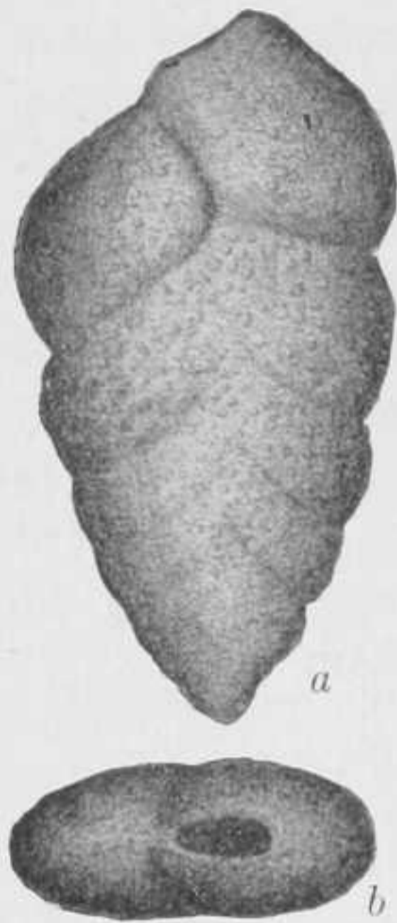
FIG. 58.—BOLIVINA COMPACTA. \times 120 . a, FRONT VIEW; b, END VIEW.
