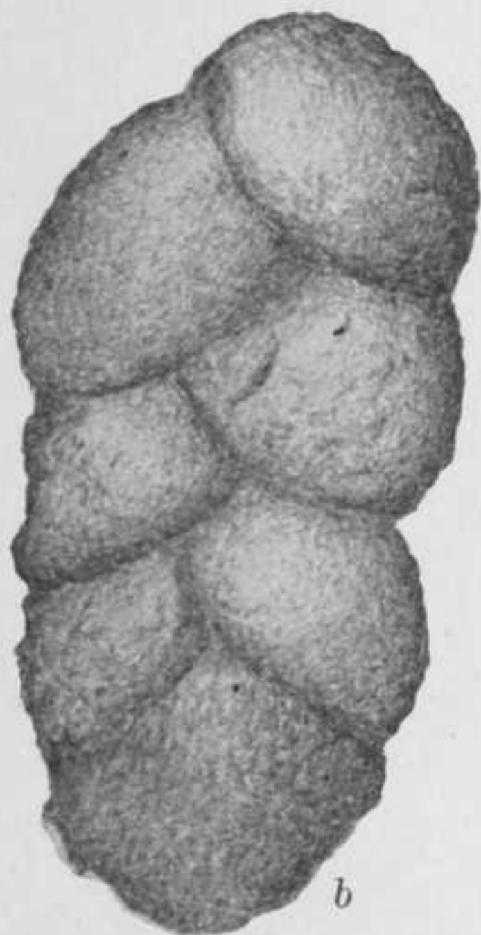
FIG. 100.—GAUDRYINA SCABRA. \times 45 . a, APERTURAL VIEW; b, FRONT VIEW.
