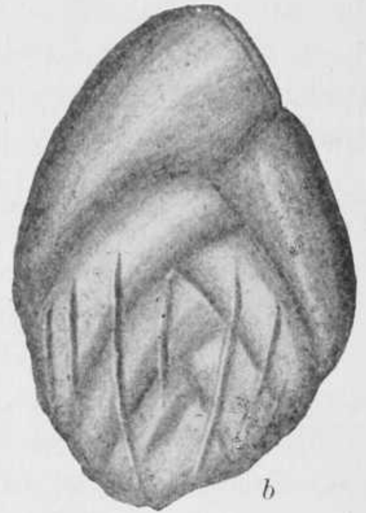
FIG. 70.— BOLIVINA SEMICOSTATA . × 75. a , APERTURAL VIEW; b , FRONT VIEW.
