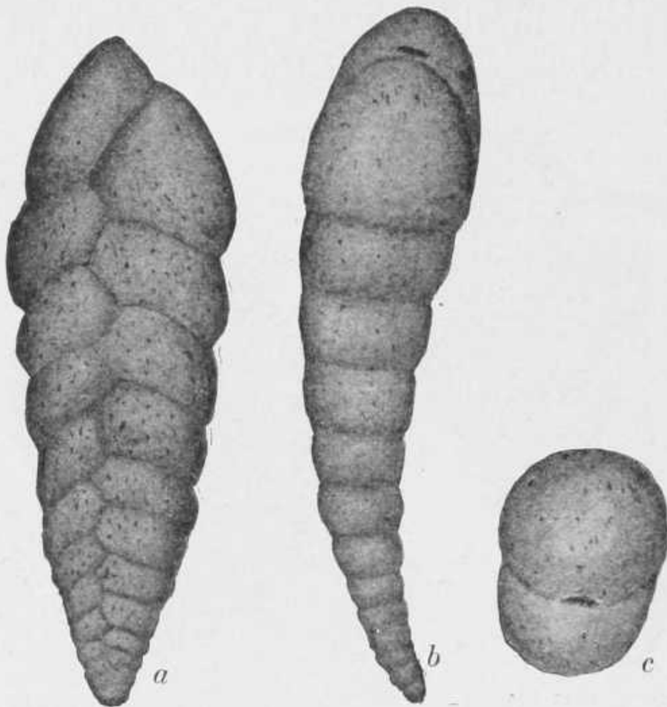
FIG. 37.— TEXTULARIA CRESCENTIFORMIS . \times 75 . a , FRONT VIEW; b , SIDE VIEW, SHOWING THE DISTINCT CURVATURE OF THE TEST; c , APERTURAL VIEW.
