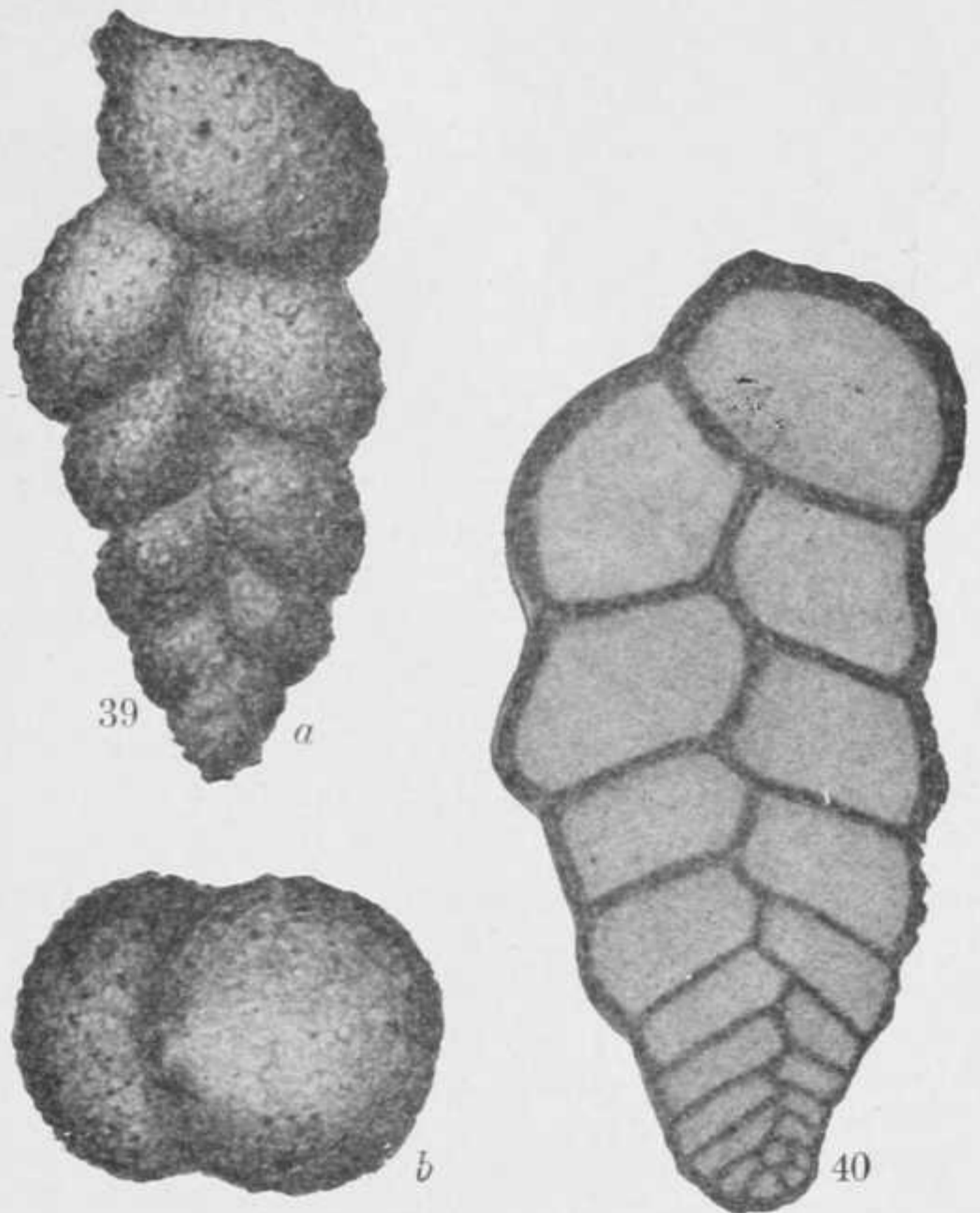
FIGS. 39–40.— TEXTULARIA CATENATA . 39, a , FRONT VIEW; b , APERTURAL VIEW. \times 60 . 40, ANOTHER SPECIMEN, MICROSPHERIC, BY TRANSMITTED LIGHT, SHOWING THE MICROSPHERIC PROLOCULUM FOLLOWED BY FOUR CHAMBERS IN A COIL BEFORE THE BISERIAL CONDITION IS TAKEN ON. \times 120 .
