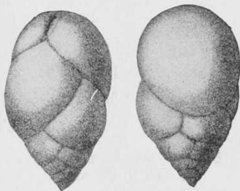
FIG. 130.— BULIMINA AFFINIS . \times 50 (AFTER BRADY).
