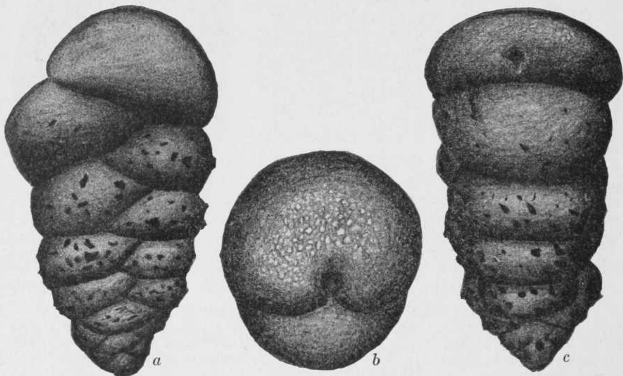
FIG. 102.—GAUDRYINA FLINTH. \times 20 . a, FRONT VIEW; b, APERTURAL VIEW; c, SIDE VIEW.
