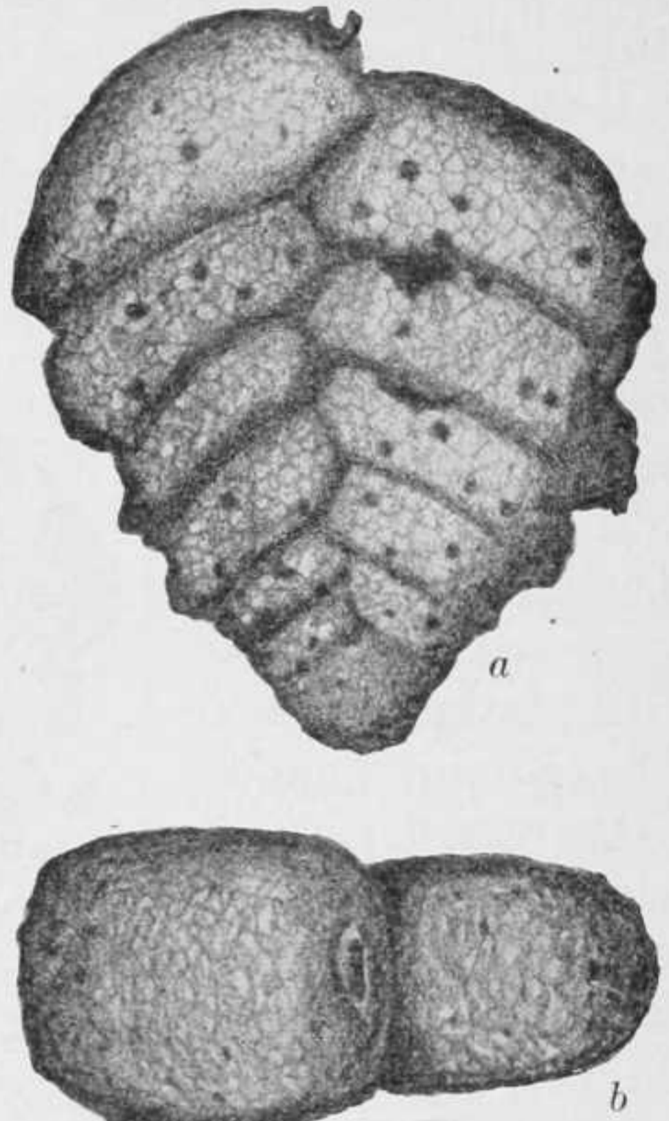
FIG. 38.— TEXTULARIA CONCAVA . \times 60 . a , FRONT VIEW; b , APERTURAL VIEW.
