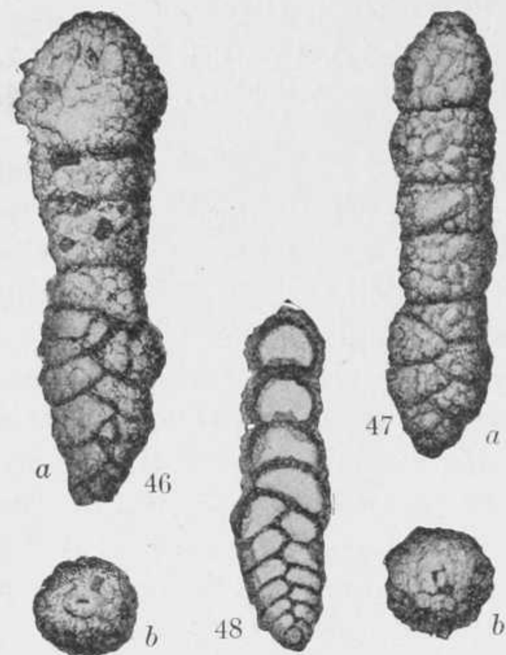
FIGS. 46-48.—BIGENERINA NODOSARIA. \times 35 . 46, a , FRONT VIEW; b , END VIEW. 47, a , FRONT VIEW; b , END VIEW. 48, LONGITUDINAL SECTION OF THE TEST (AFTER BRADY).
