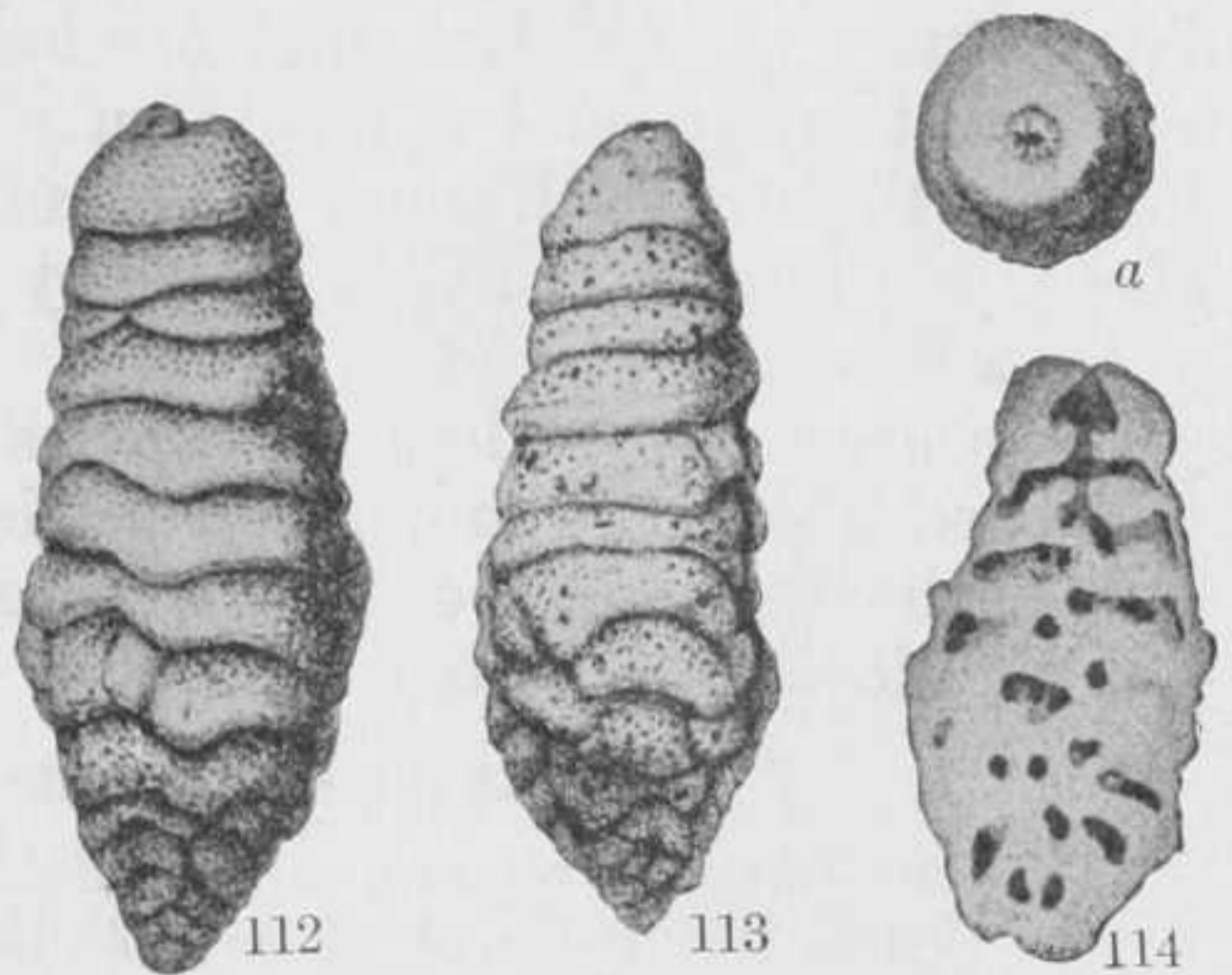
FIGS. 112-114.—TRITAXILINA CAPERATA. \times 16 . 112, a, APERTURAL VIEW. 114, SPECIMEN CUT LONGITUDINALLY, SHOWING LABYRINTHIC INTERIOR (AFTER BRADY).
