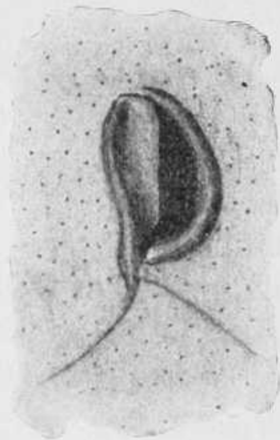
FIG. 127.—BULIMINA PYRULA. \times 75 . DETAILS OF THE APERTURE.
