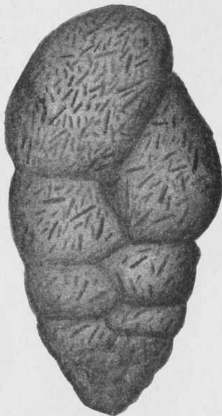
FIG. 101.—GAUDRYINA SCABRA. \times 30 SPECIMEN WITH WALL CONTAINING SPONGE SPICULES.
