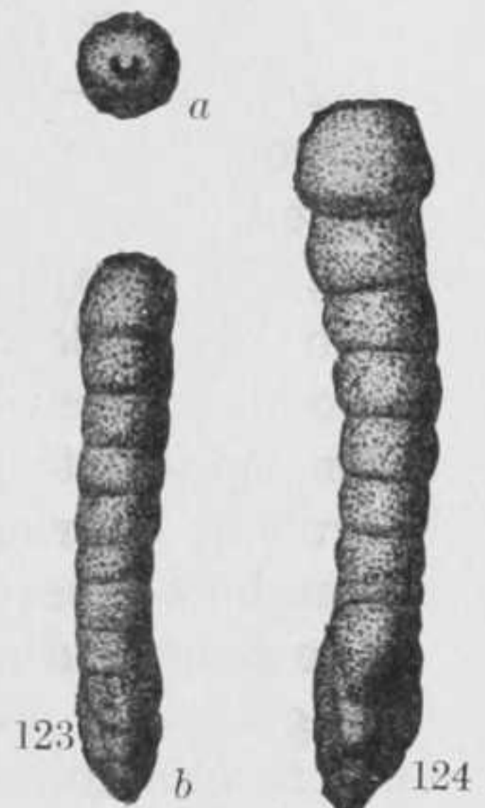
FIGS. 123-124.—CLAVULINA PARISIENSIS. \times 30 . 123, a, APERTURAL VIEW; b, FRONT VIEW (AFTER BRADY).
